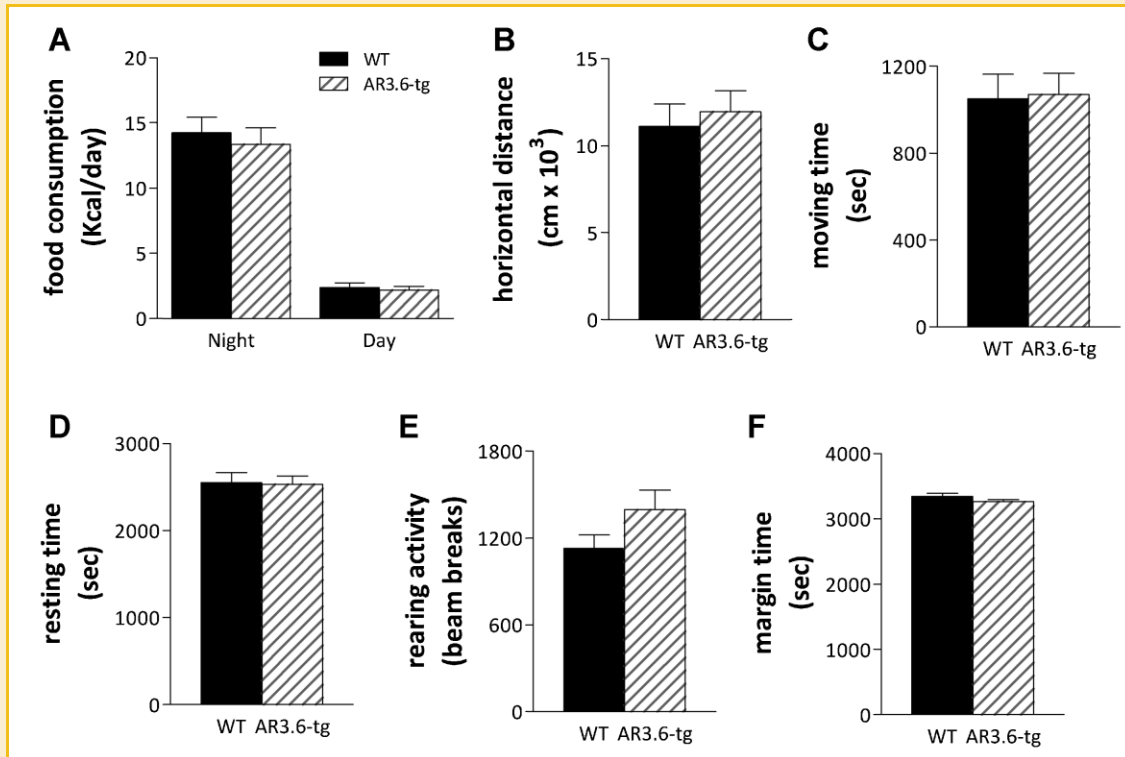
Fig. 3. No differences in food intake or baseline locomotor activity in AR transgenic mice. A: Food consumption for WT and AR3.6-tg male mice ( n = 8-9 ) was determined overnight ( \sim 16 h) and during each day ( \sim 8 h) for five consecutive days. Data are shown in kcal/day as mean \pm SEM. No significant differences between the genotypes were noted. Spontaneous locomotor activity shown as (B). horizontal distance, (C). total time moving, (D). total time resting, (E). rearing activity, and (F). margin time (thigmotaxis). Data presented as mean \pm SEM; n = 12 per genotype. No significant differences were observed between the genotypes.
